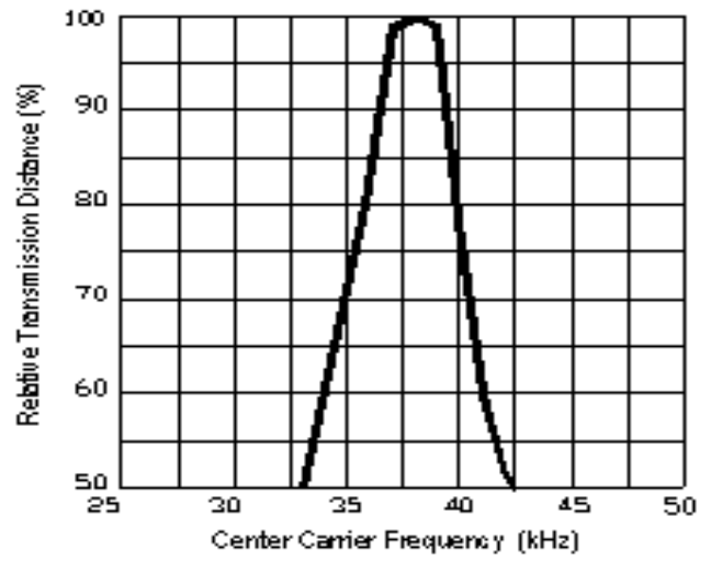
Fig.-9 Relative Transmission Distance vs. Center Carrier Frequency -IRM-2638T
