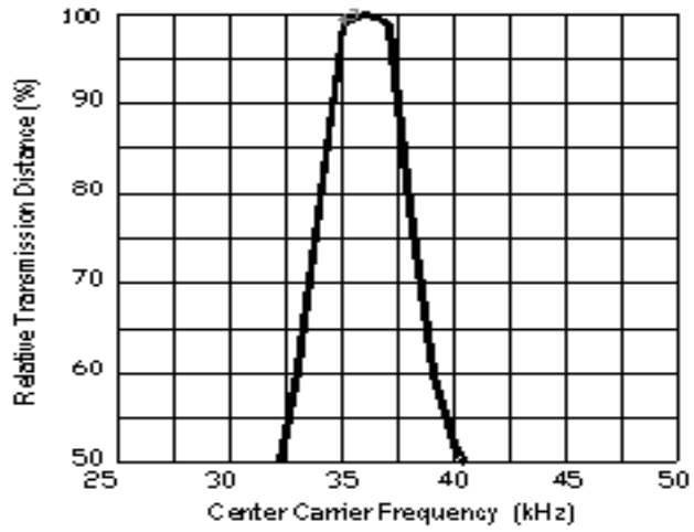
Fig.-8 Relative Transmission Distance vs. Center Carrier Frequency -IRM-2636T
