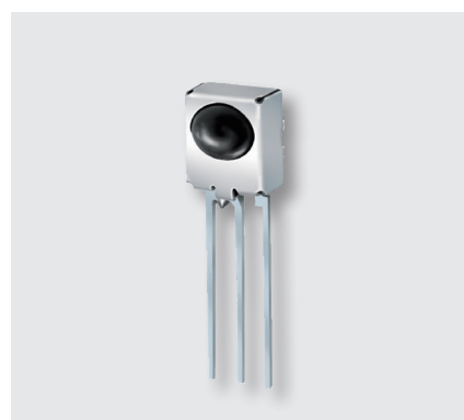
Product Dimension HxLxD (mm) Supply Voltage(V) Carrier Freq. (KHz) Supply Current Typ. (mA) Reception Range L0 Typ.(m) Half viewing angle Horizontal Typ. (degree) Reception Range L45 typ.(m) IRM-8601JF 8.95x6.8x6 4.5~5.5 36/38/40 0.48 8 ±45 5
