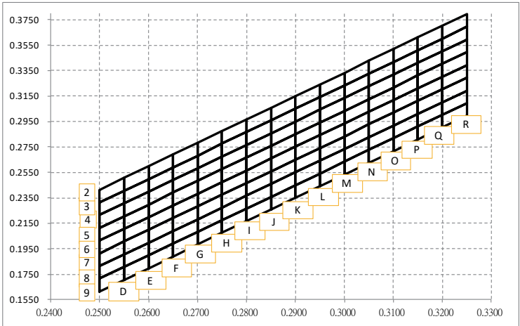
Chromaticity Diagram
